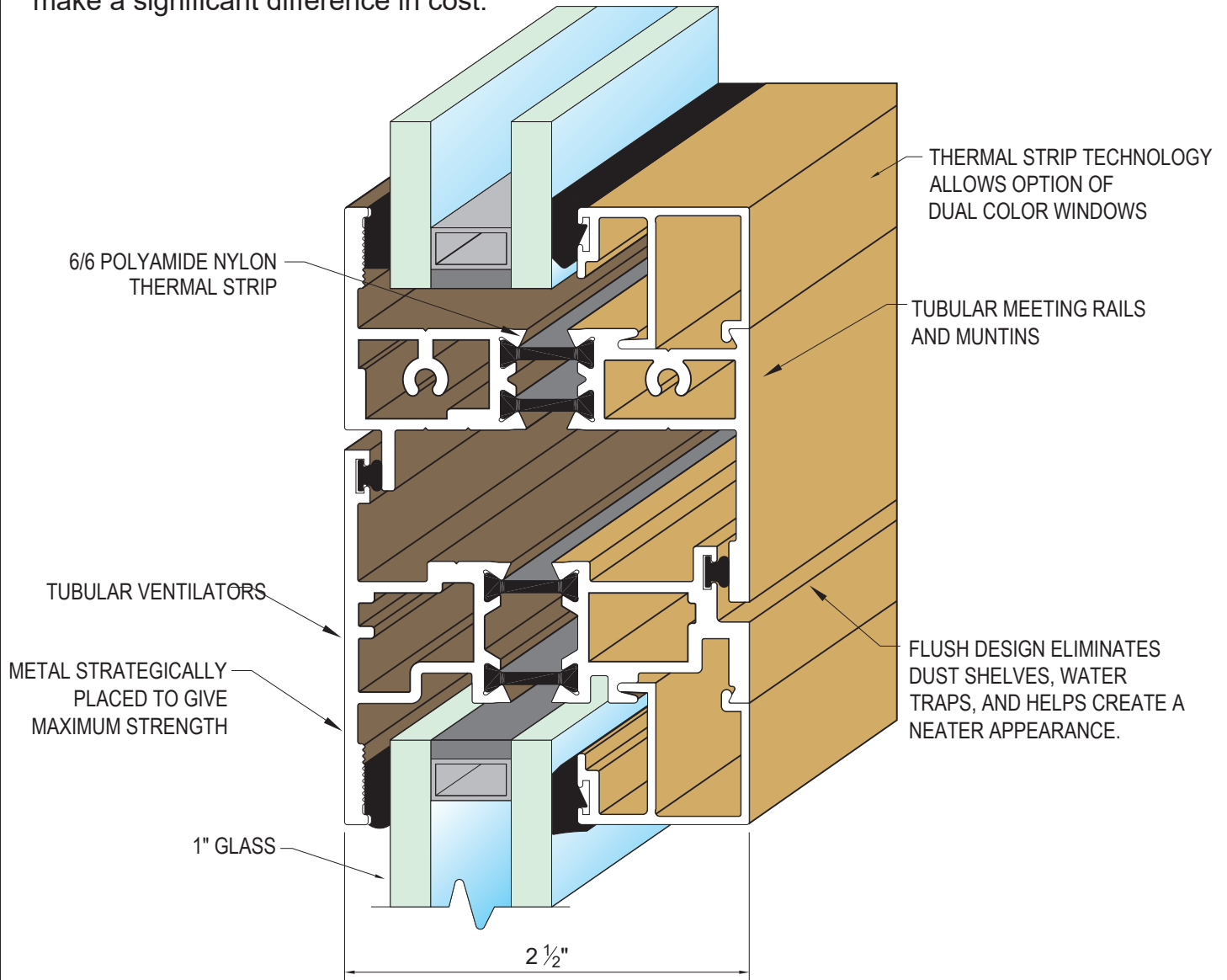
SCALE = FULL SIZE
