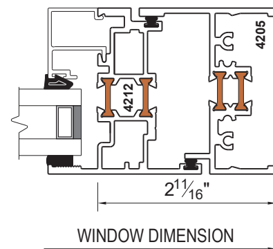
5 ALTERNATE JAMB DEPENDING ON SIZE AND CONFIGURATION (Consult Factory)
