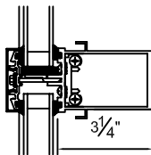
CROSS BAR
