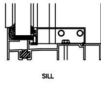
SILL
