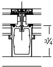
RAFTER
