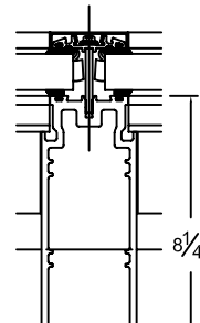
RAFTER
